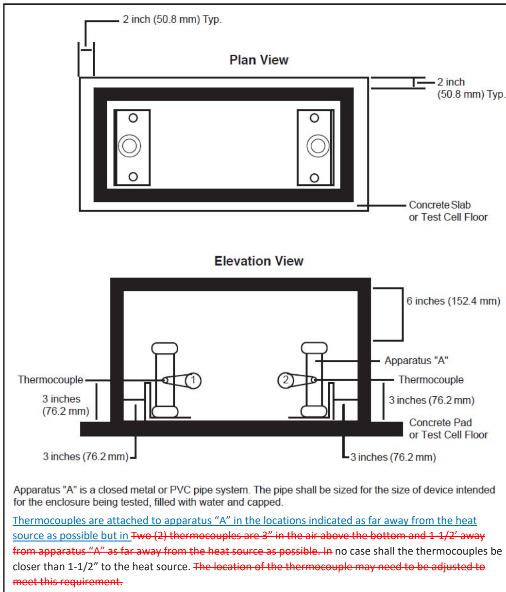
Figure 3 Thermocouple Placement
