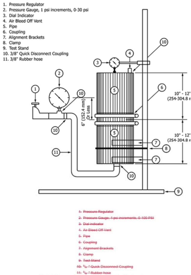
FIG. 3 Unrestrained Hydrostatic Joint Testing Apparatus
