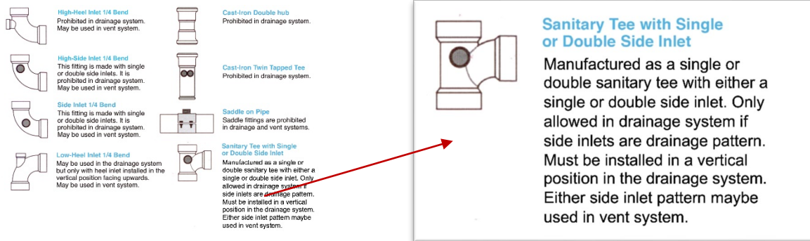
FIGURE 310.1 PROHIBITED OR RESTRICTED FITTINGS
